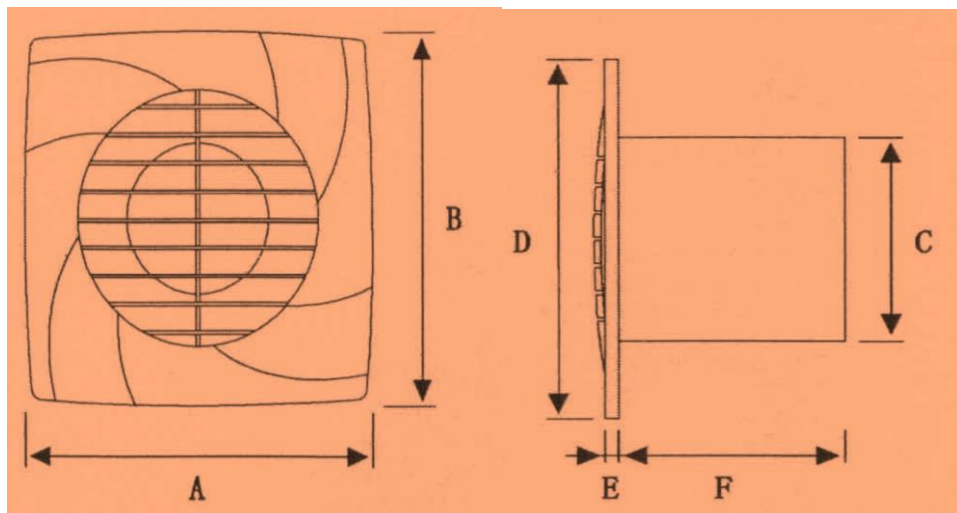
Dimension details:-
